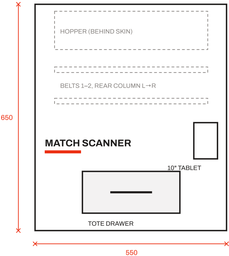
FRONT — WIDTH 550
