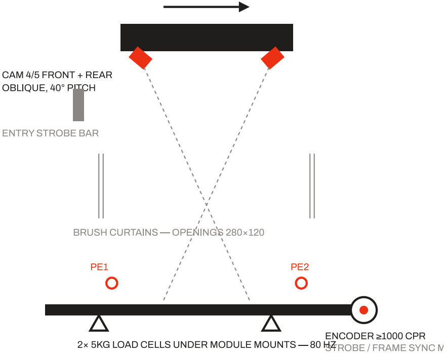
SECTION — ALONG BELT (TRAVEL →)
