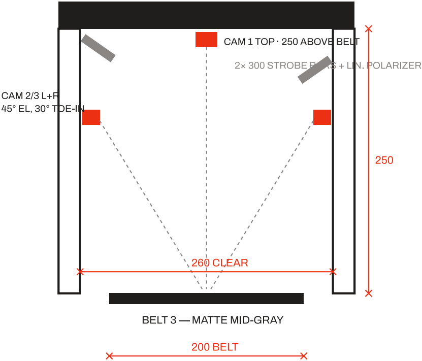
SECTION — LOOKING ALONG TRAVEL
