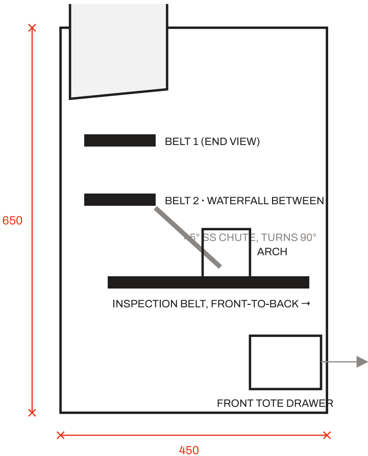
SIDE — DEPTH 450 (REAR ← → FRONT) LIFT-OFF HOPPER, TOP REAR
